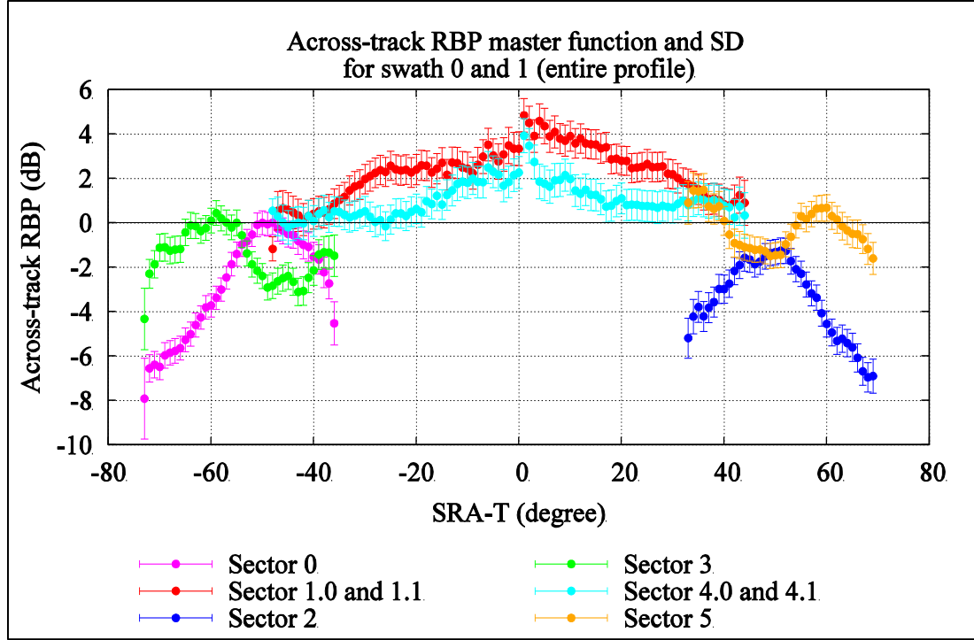
Figure 4.33: Across-track RBP master function in dB
