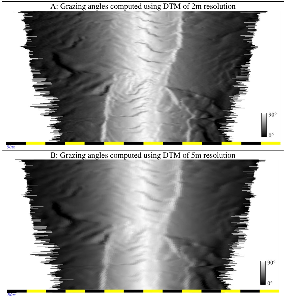
Figure 4.9: GRAs computed using different DTMs
