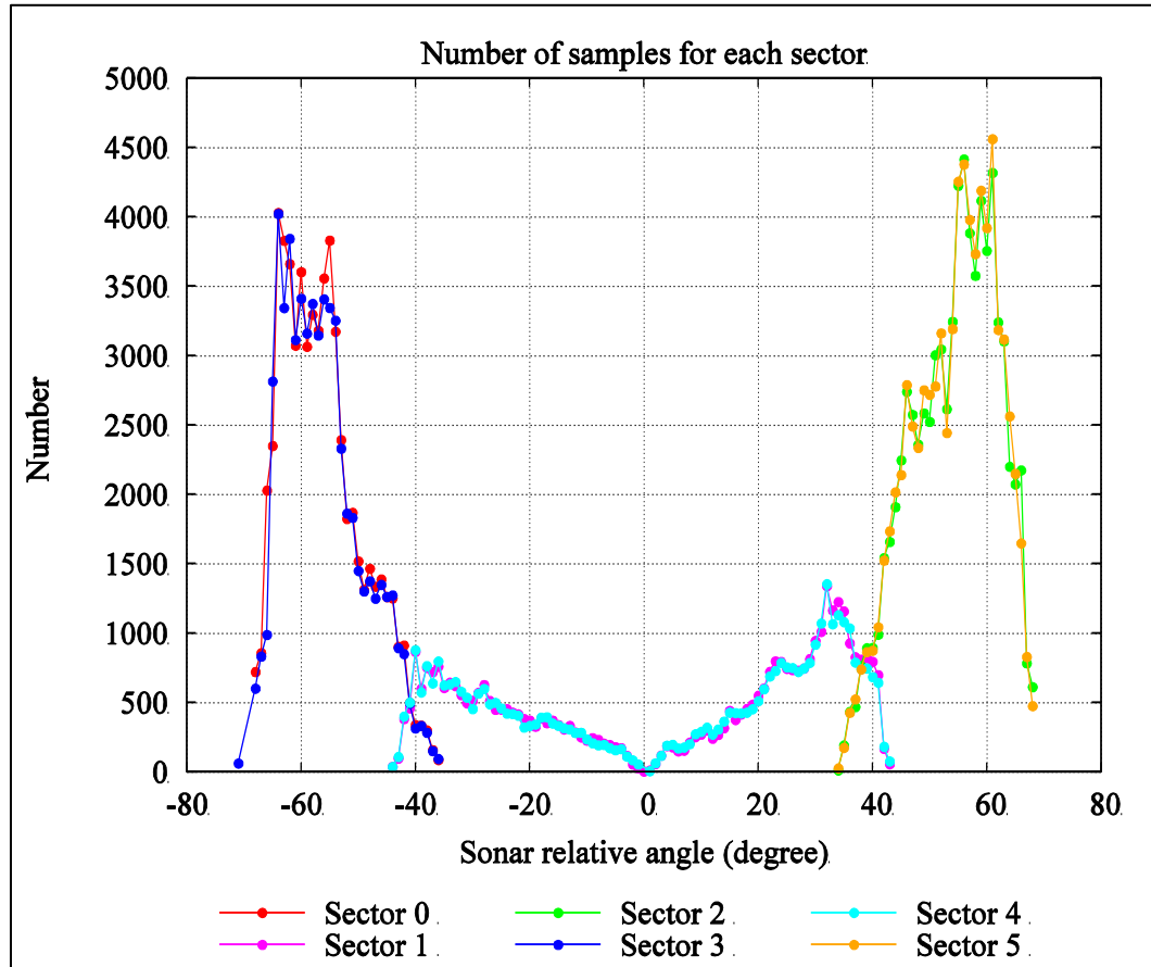
Figure 4.17: Sector-specific number of samples after sorting the backscatter data
