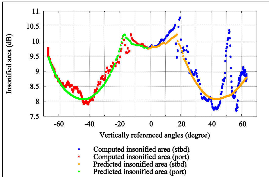
Figure 4.2: Magnitude of insonified area correction for a single profile on undulating seafloor
