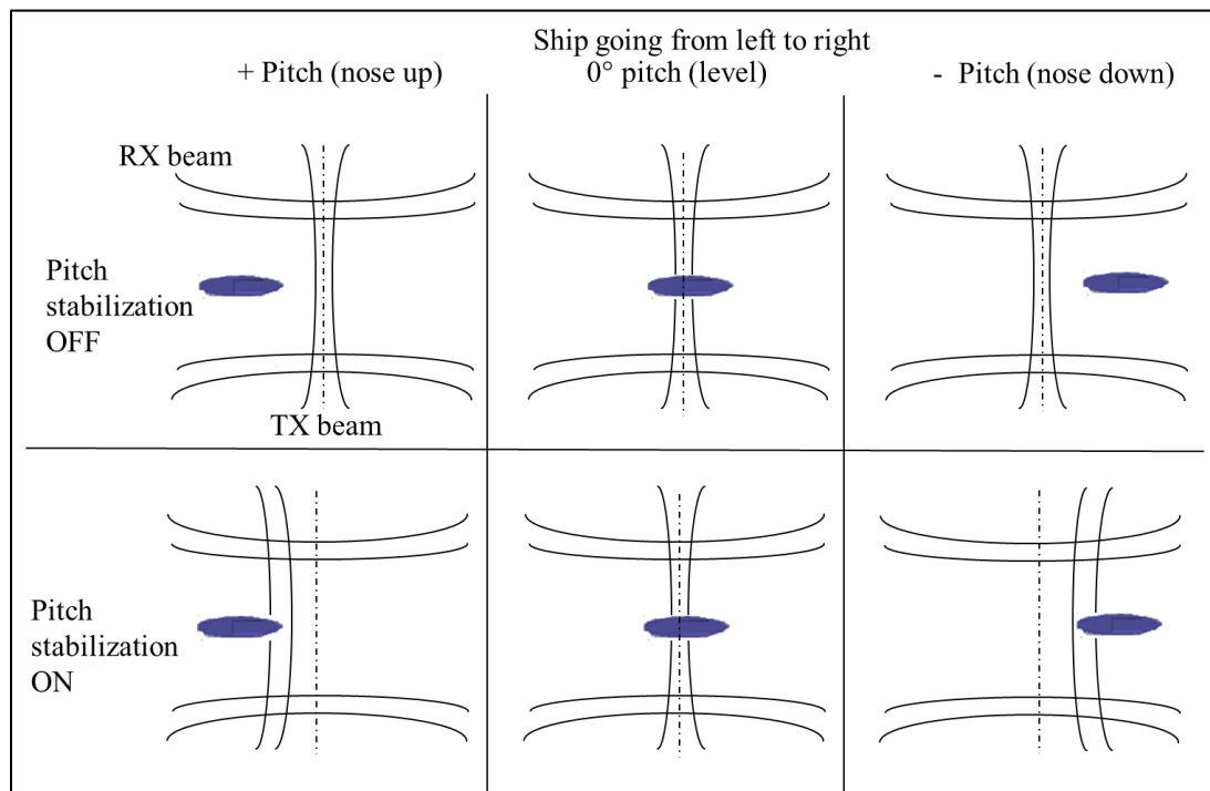
Figure 3.7: Transmit and receive beam geometry and pitch stabilization (dotted lines shows peak response of unsteered Tx and Rx beams).
