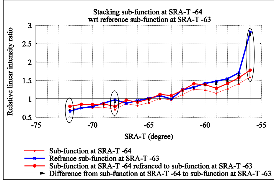
Figure 4.19: Stacking process for sub-function at SRA-T -64^\circ wrt sub-function at SRA-T -63^\circ . Circled values were detected as outliers
