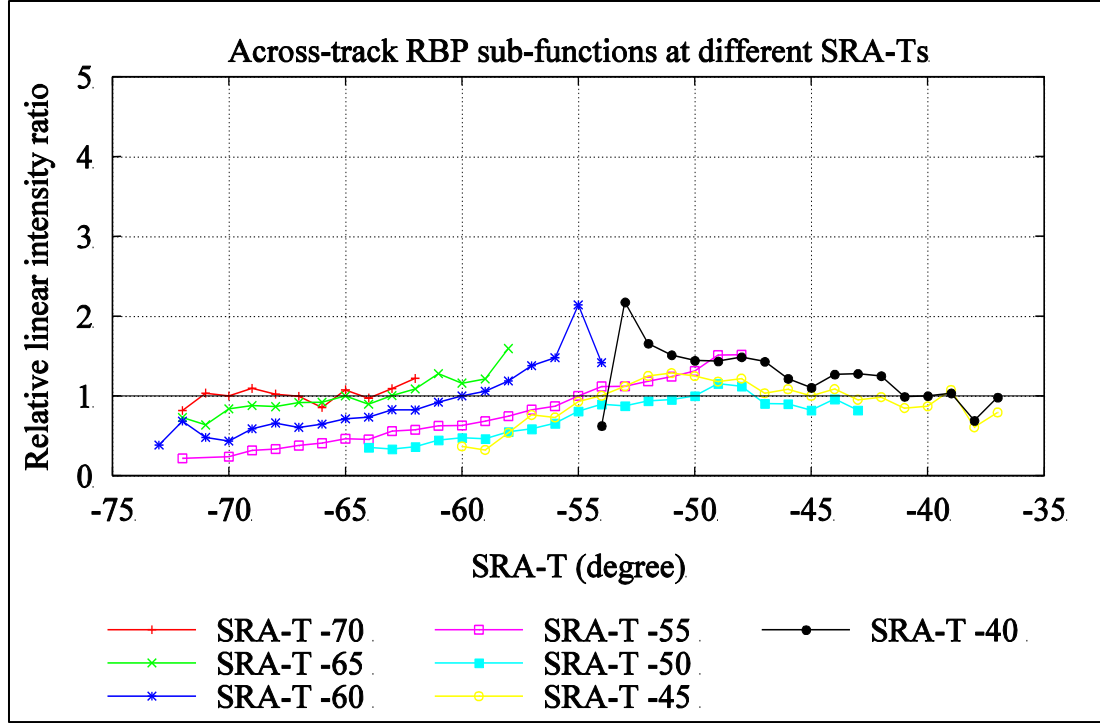
Figure 4.16: Few across-track RBP sub-functions from sector 0 with individual reference SRA-T. The ratio at the reference is 1.
