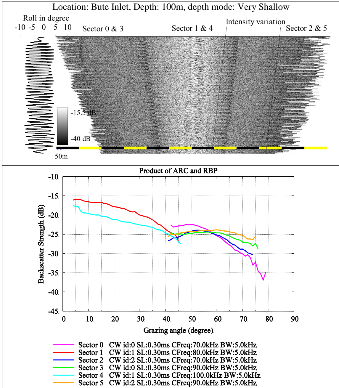
Figure 4.3: TVG-BS-free backscatter intensities for across-track RBP extraction with the product of ARC and RBP from test survey line collected in Bute Inlet
