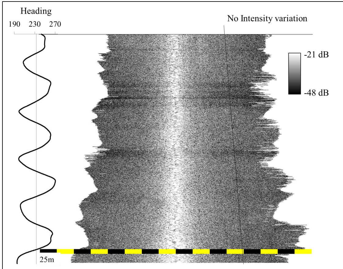
Figure 4.48: Along- and across-track RBP free backscatter intensities
