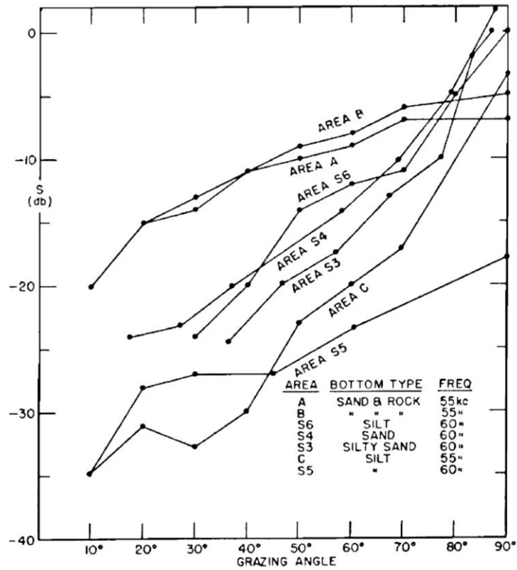
Figure 1.1: Scattering strength as a function of grazing angle at 55 and 60 kHz by Urick [1954]
