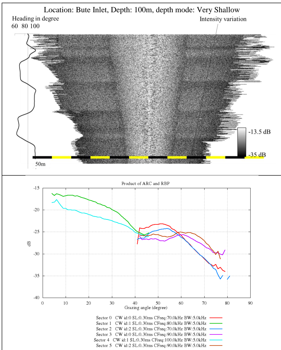
Figure 4.5: TVG-BS-free backscatter intensities for along-track RBP extraction with the product of ARC and RBP from test survey line collected in Bute Inlet
