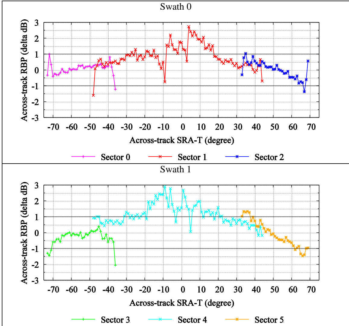
Figure 6.14: Differences between 2014 and 2015 across-track RBPs
