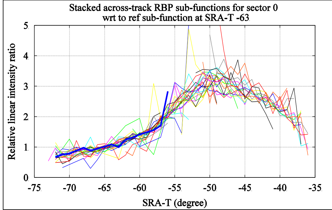
Figure 4.22: Stacked sub-functions for entire sector 0 wrt reference sub-function at SRA-T -63° shown in dark blue
