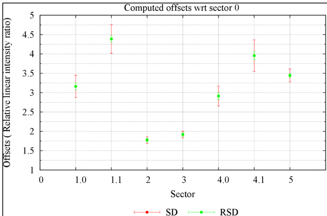
Figure 4.30: Final computed offsets from reference sector 0 and related SD
