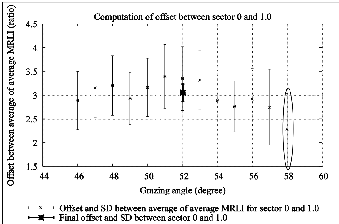
Figure 4.29: Computation of single offset between sector 0 and sector 1.0 by averaging multiple offsets as a result of overlapping GRAs.
