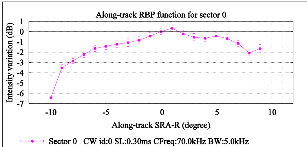
Figure 4.45: Final along-track RBP function with SD for sector 0 in dB
