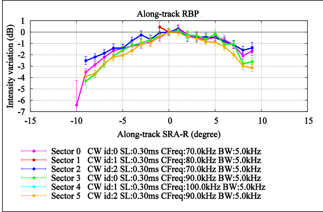
Figure 4.46: Final along-track RBP function with SDs for all sectors in dB
