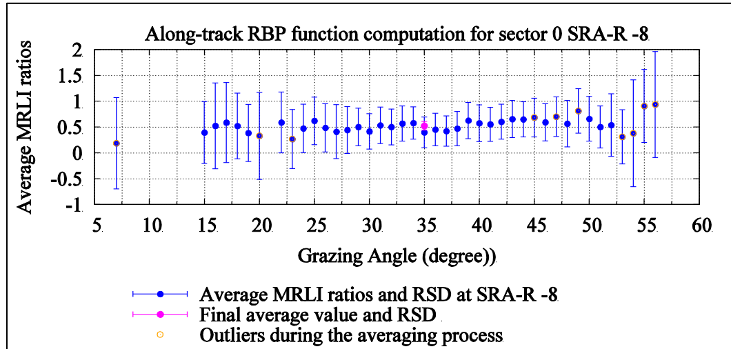
Figure 4.43: Computation of along-track RBP function value at SRA-R -8^{\circ} by averaging sub-function values from all possible GRAs
