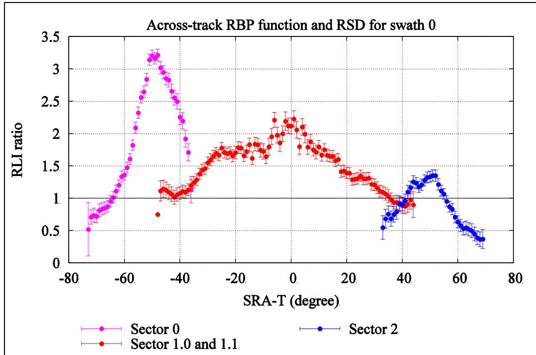
Figure 4.24: Average Across-track RBP function for all sectors in swath 0 referenced to respective sector-specific SRA-T
