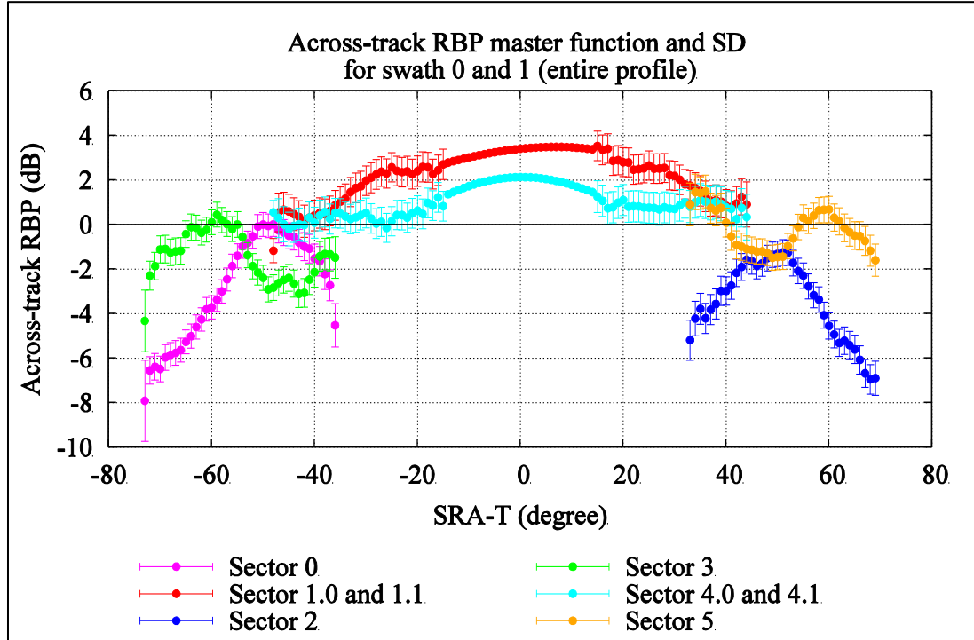
Figure 4.34: Across-track RBP master function with interpolated values at nadir
