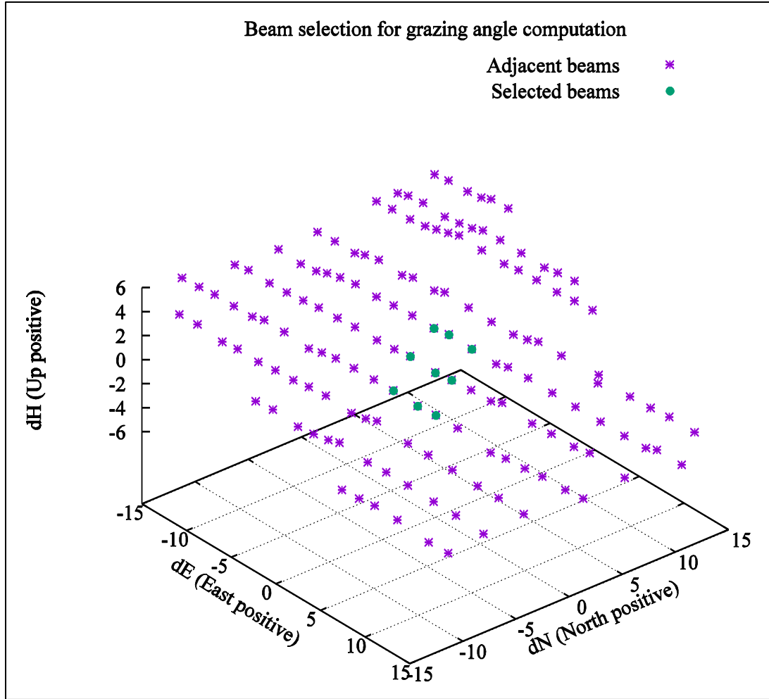
Figure 4.7: Selected 9 beams for least square plane fitting to compute GRA at the central selected beam.
