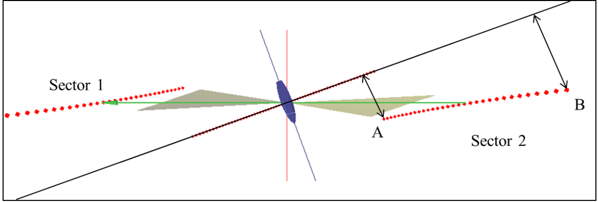
Figure 4.10: Circular projection of detected beams due to steered Tx sectors and Rx beams
