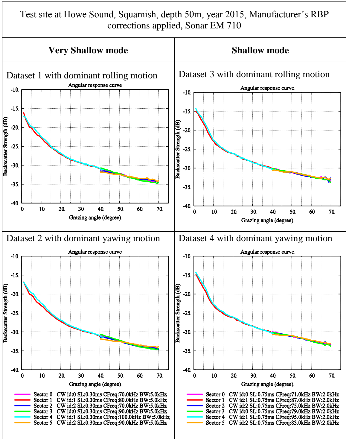
Figure 6.6: ARCs obtained after removing extracted RBPs for datasets 1, 2, 3, and 4
