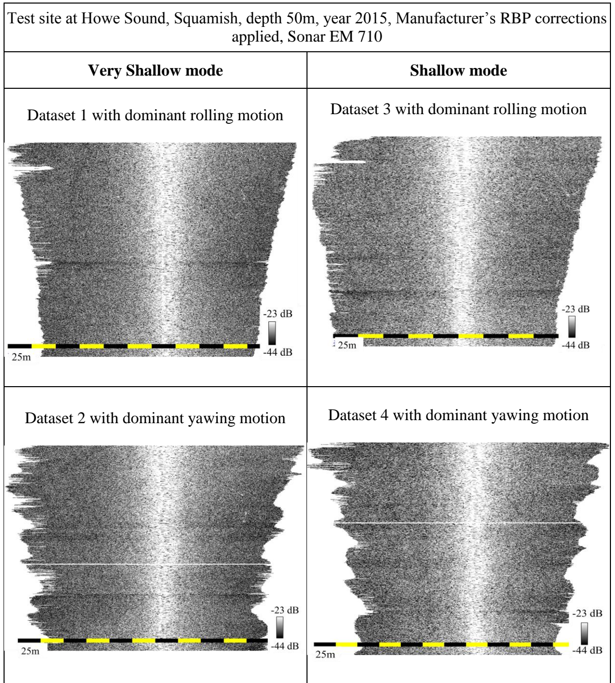
Figure 6.4: RBP corrected backscatter intensities for all 4 cases
