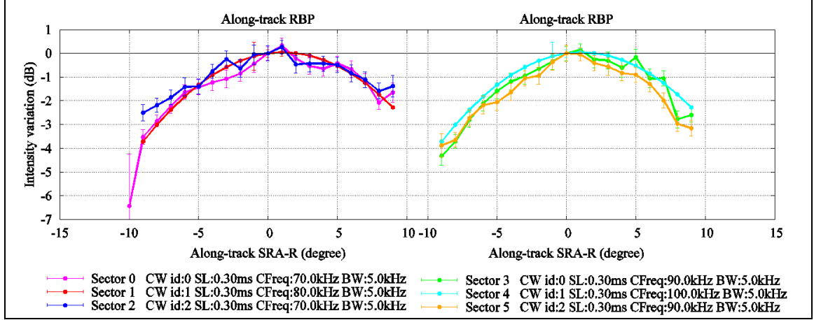
Figure 4.47: Predicted along-track RBP functions for central sector
