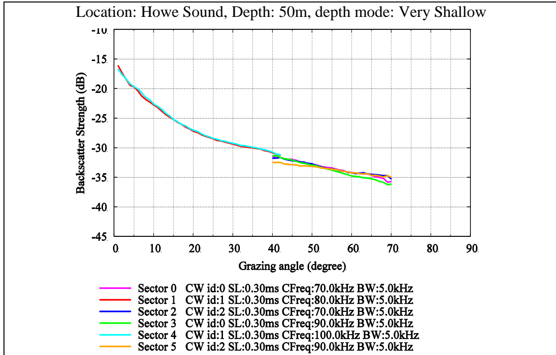
Figure 4.41: Backscatter strength curves showing product of ARC and along-track RBP
