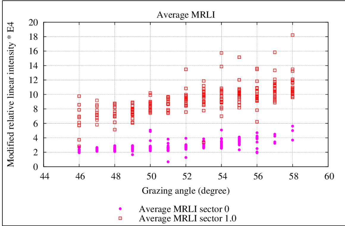
Figure 4.27: Average MRLIs for sector 0 and sector 1.0
