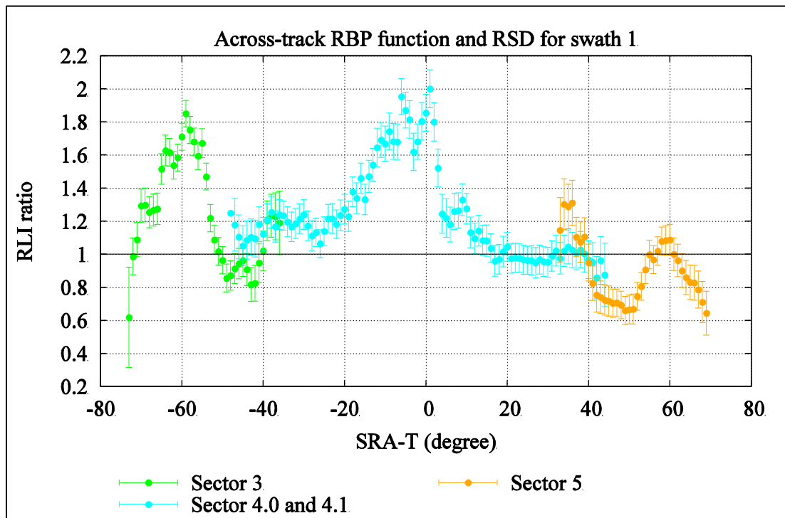
Figure 4.25: Average across-track RBP function for all sectors in swath 1 referenced to respective sector-specific SRA-T
