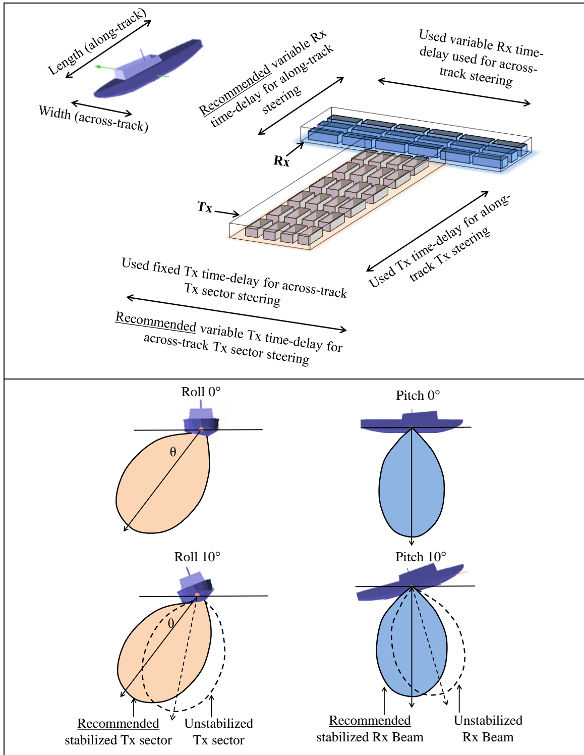
Figure 7.1: Recommended time delays for complete motion stabilization
