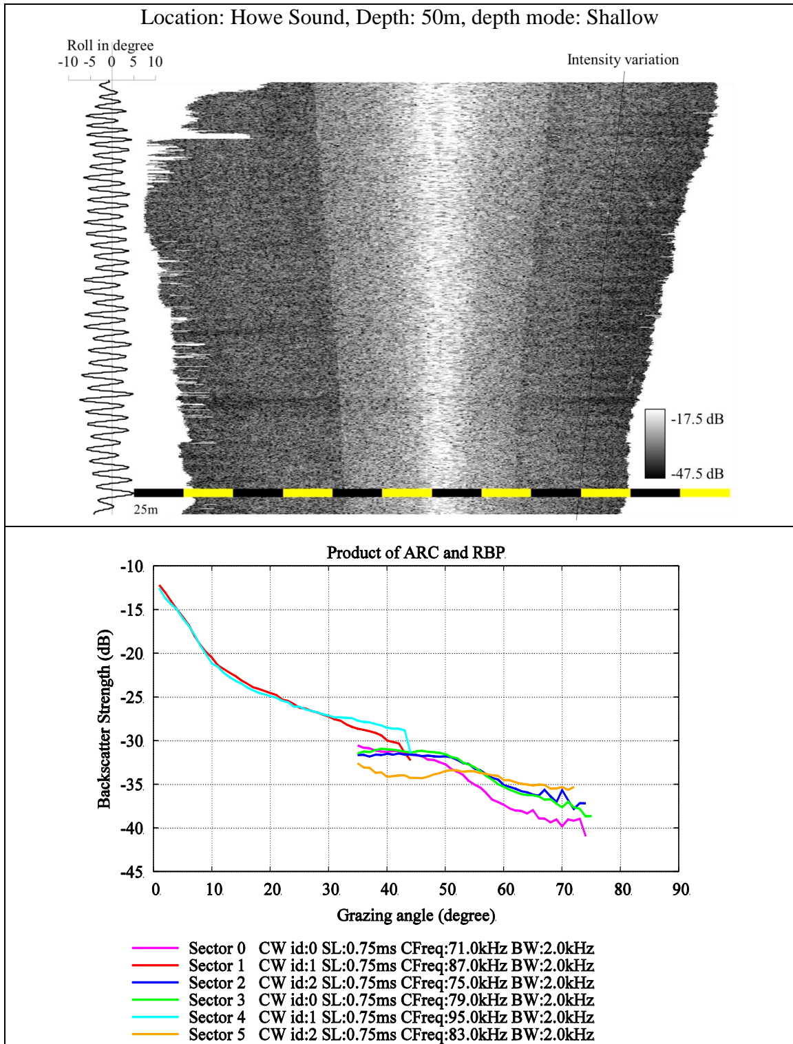
Figure 4.4: TVG-BS-free backscatter intensities for across-track RBP extraction with the product of ARC and RBP from test survey line collected in Howe Sound (Squamish)
