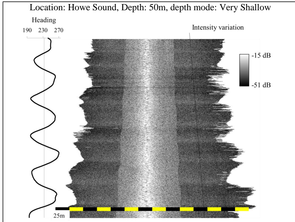
Figure 4.38: TVG-BS-free backscatter intensities
