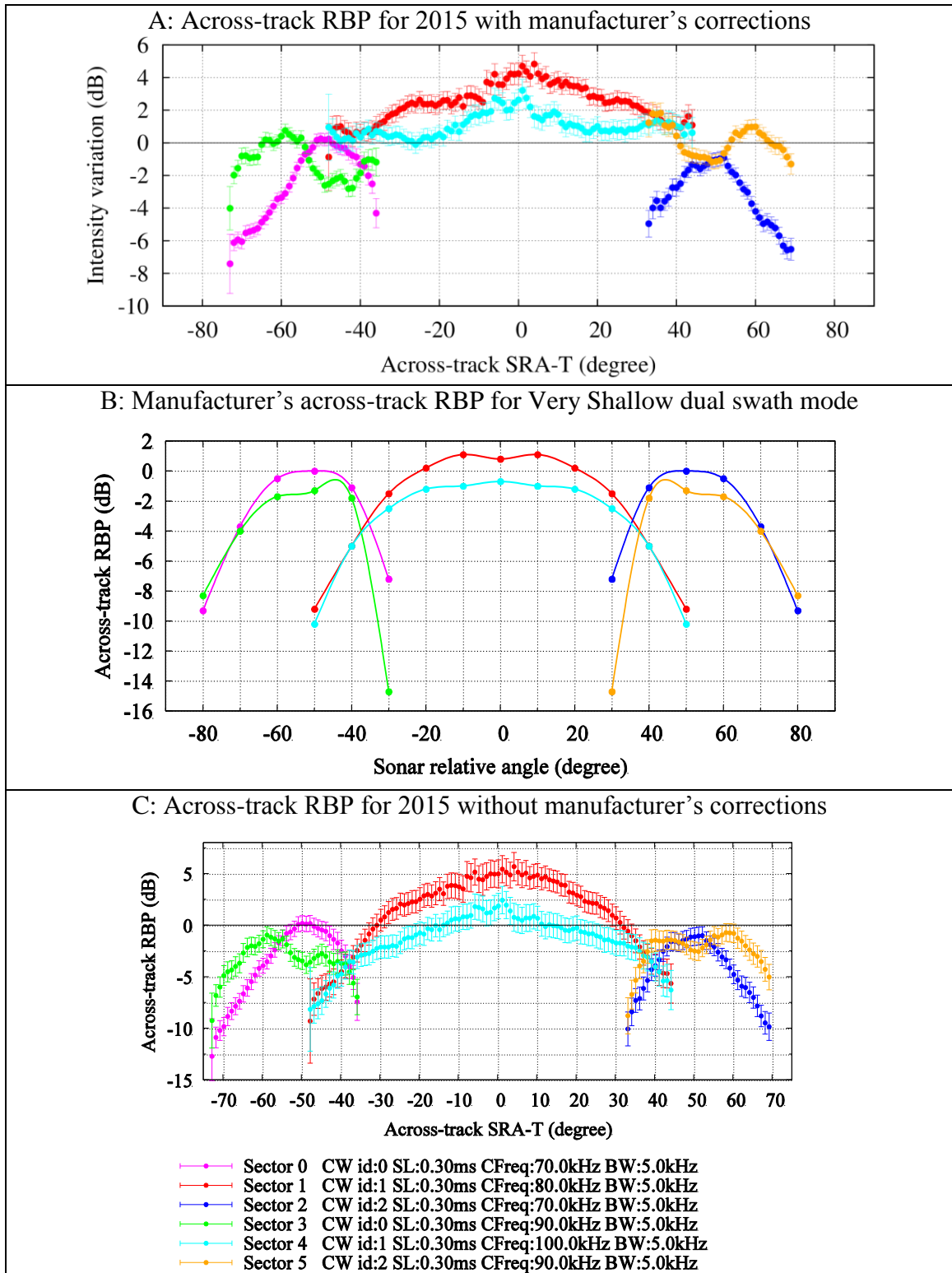
Figure 6.11: Extracted and manufacturer's across-track RBP
