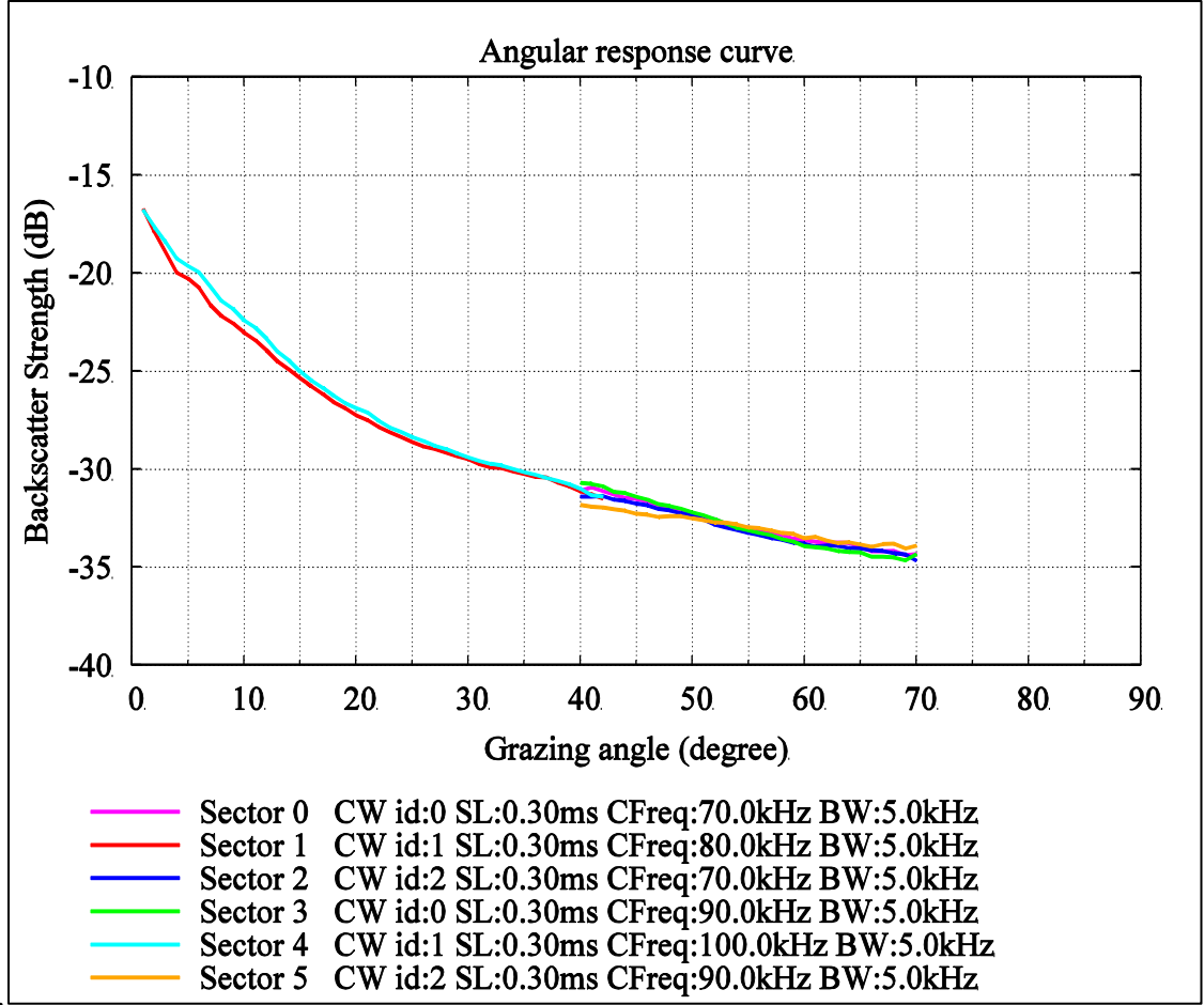
Figure 4.49: RBP-free angular response curve
