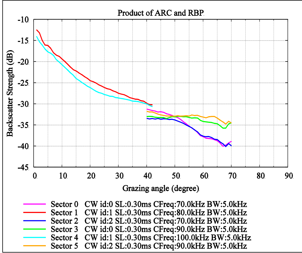
Figure 4.15: Backscatter strength curves showing product of RBP and ARC for the test dataset
