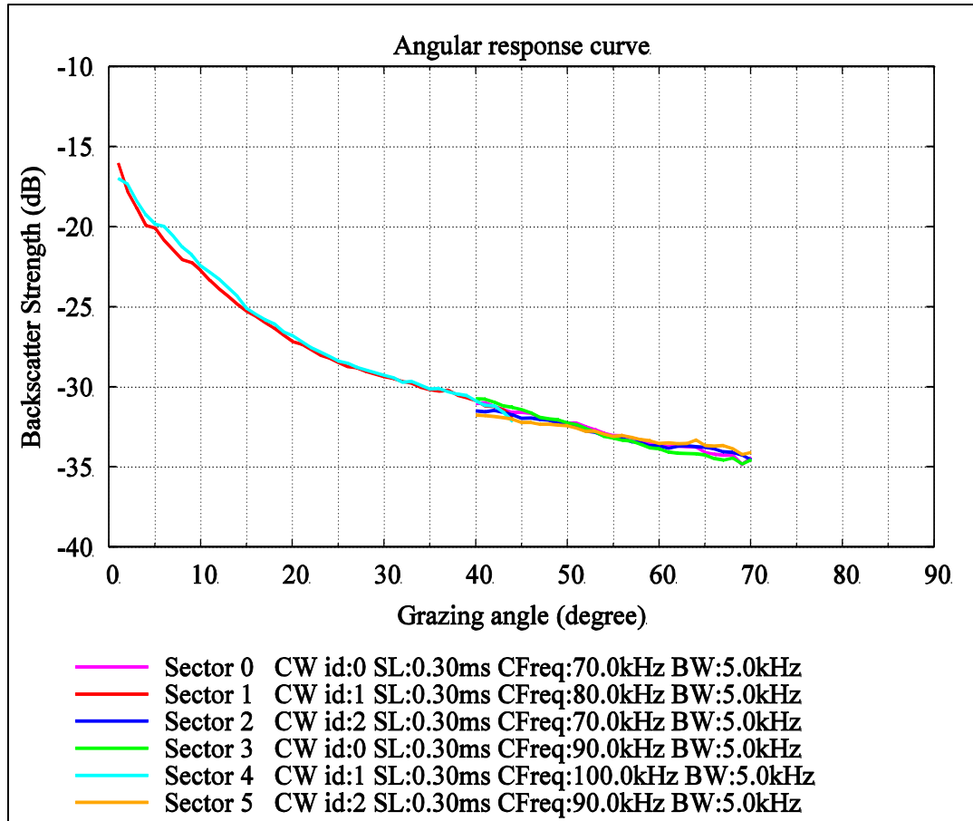
Figure 4.35: Across-track RBP-free ARC for the test dataset
