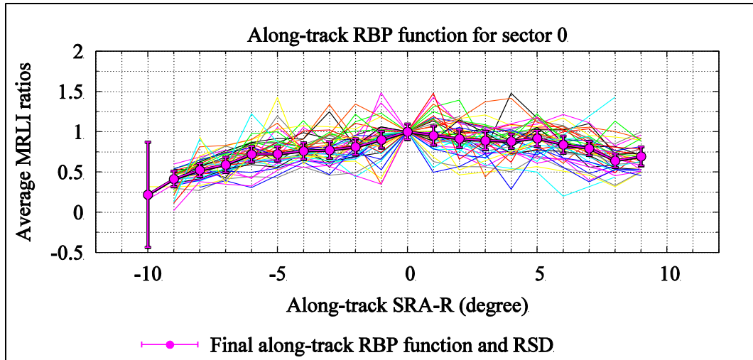
Figure 4.44: Final along-track RBP function with RSDs for sector 0
