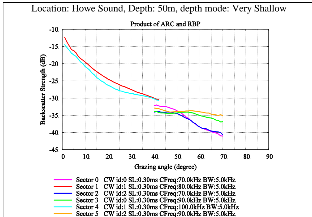
Figure 4.39: Backscatter strength curves showing product of ARC and RBP
