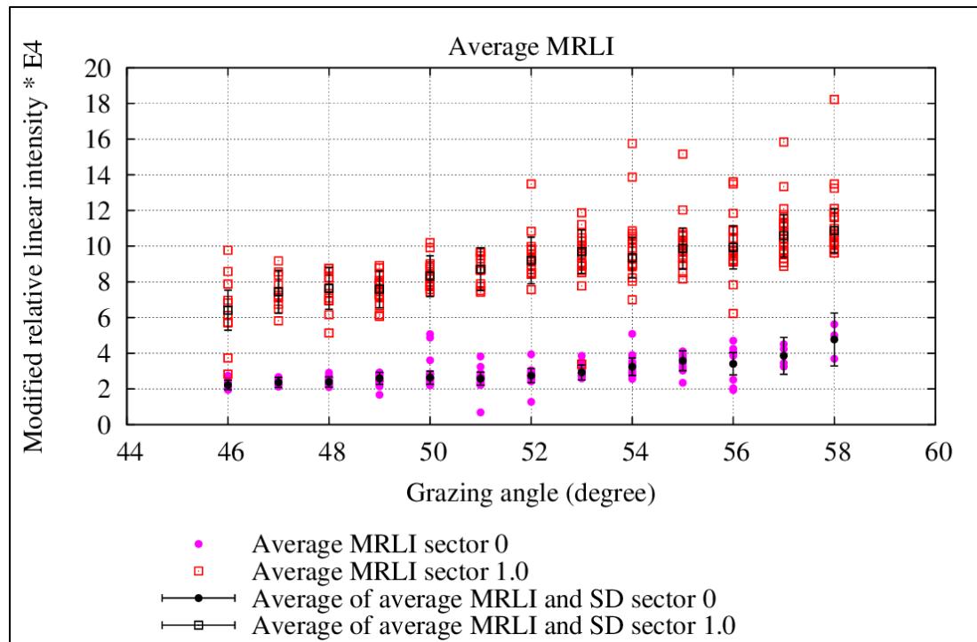
Figure 4.28: Computation of average of average MRLIs and their SDs
