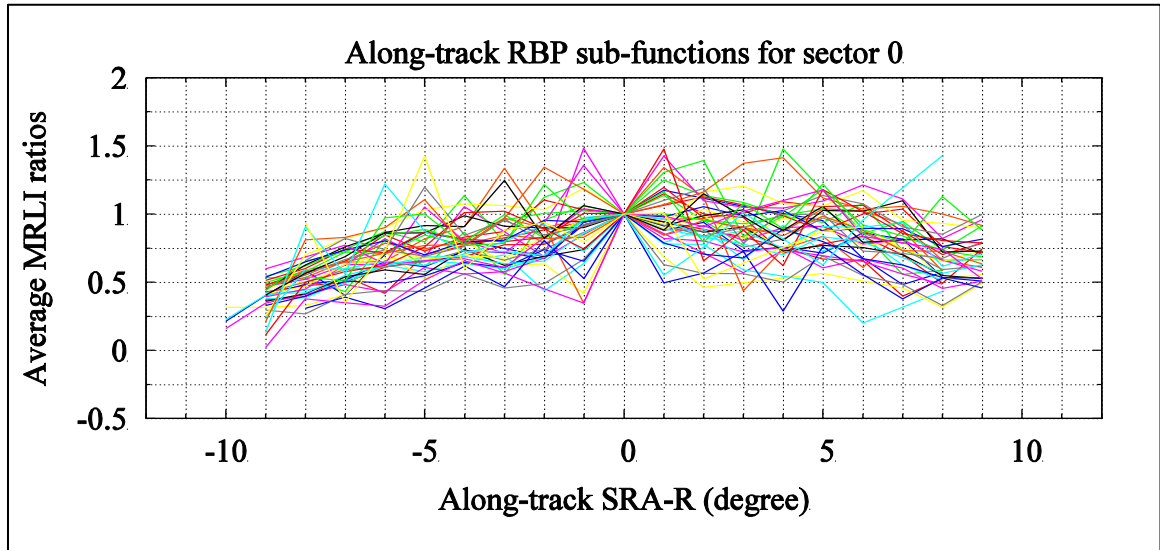
Figure 4.42: Multiple along-track RBP sub-functions for sector 0
