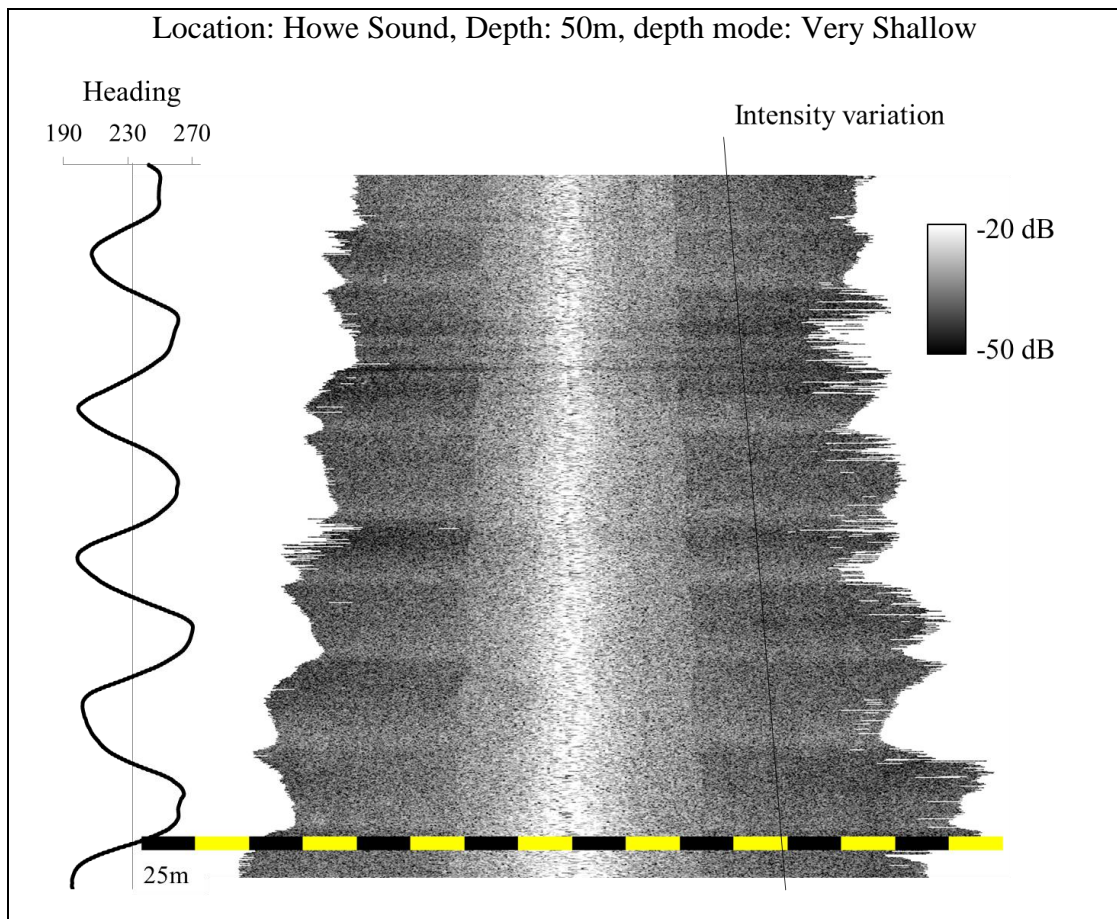
Figure 4.40: Across-track RBP free backscatter intensities
