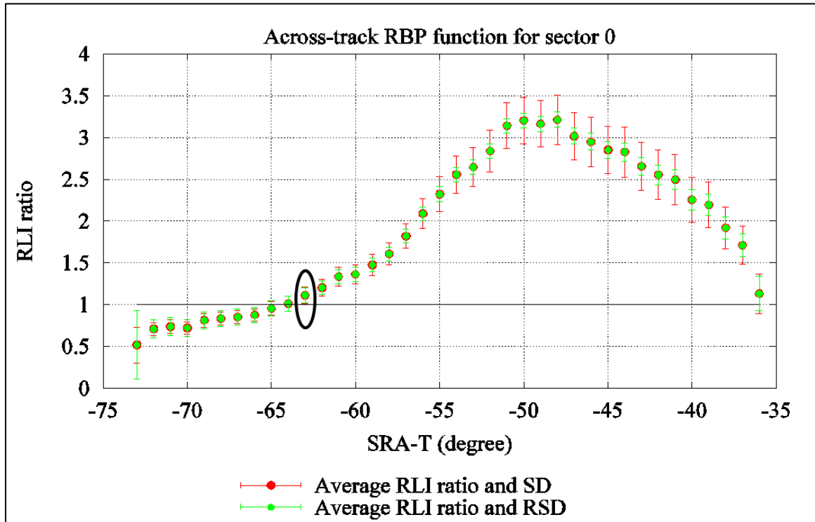
Figure 4.23: Computation of average across-track RBP function for sector 0
