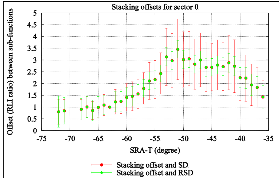
Figure 4.20: Stacking offsets and their SDs for all sub-functions of sector 0
