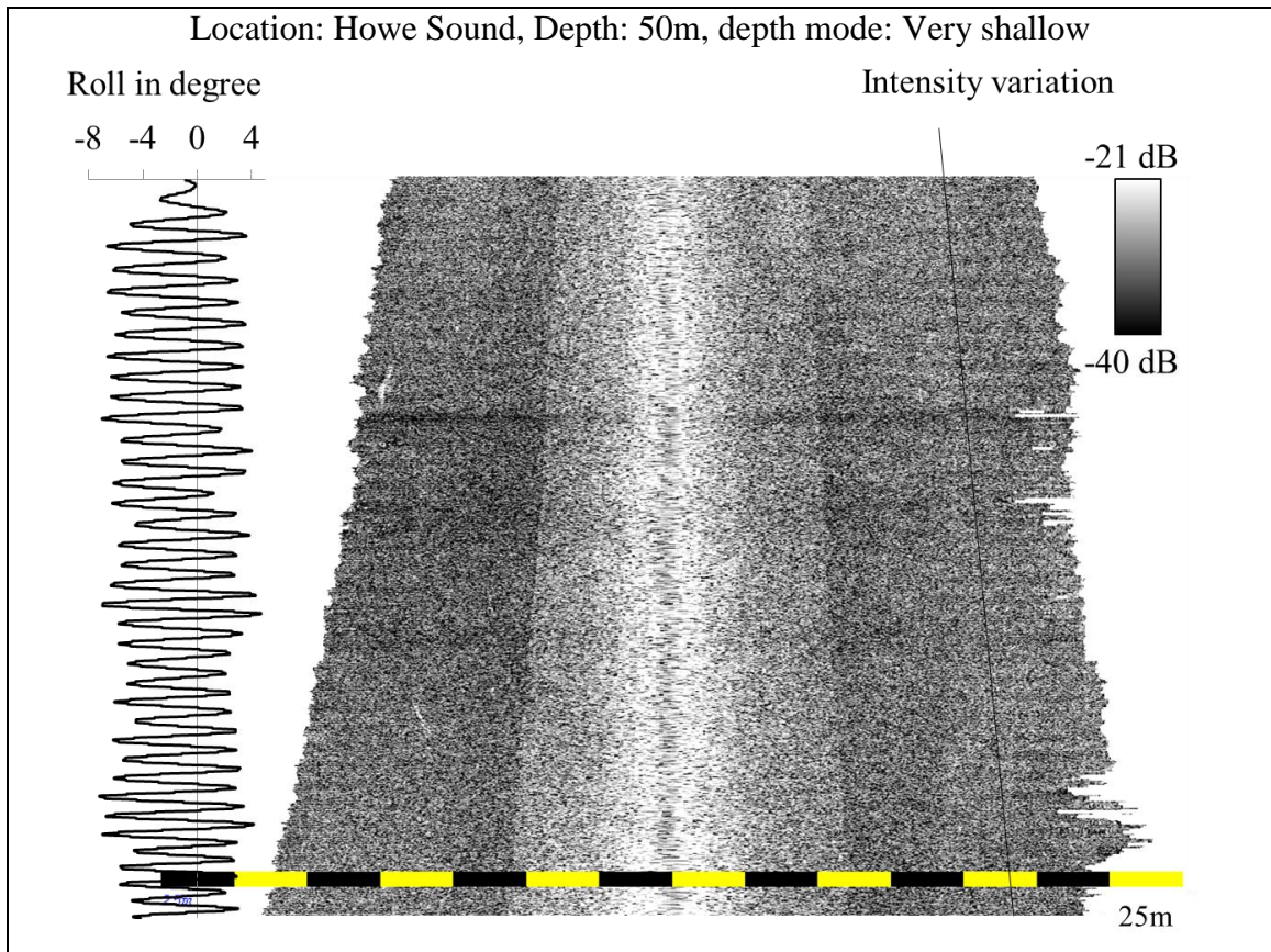
Figure 4.13: Showing received intensities for across-track RBP extraction from one of the test survey lines
