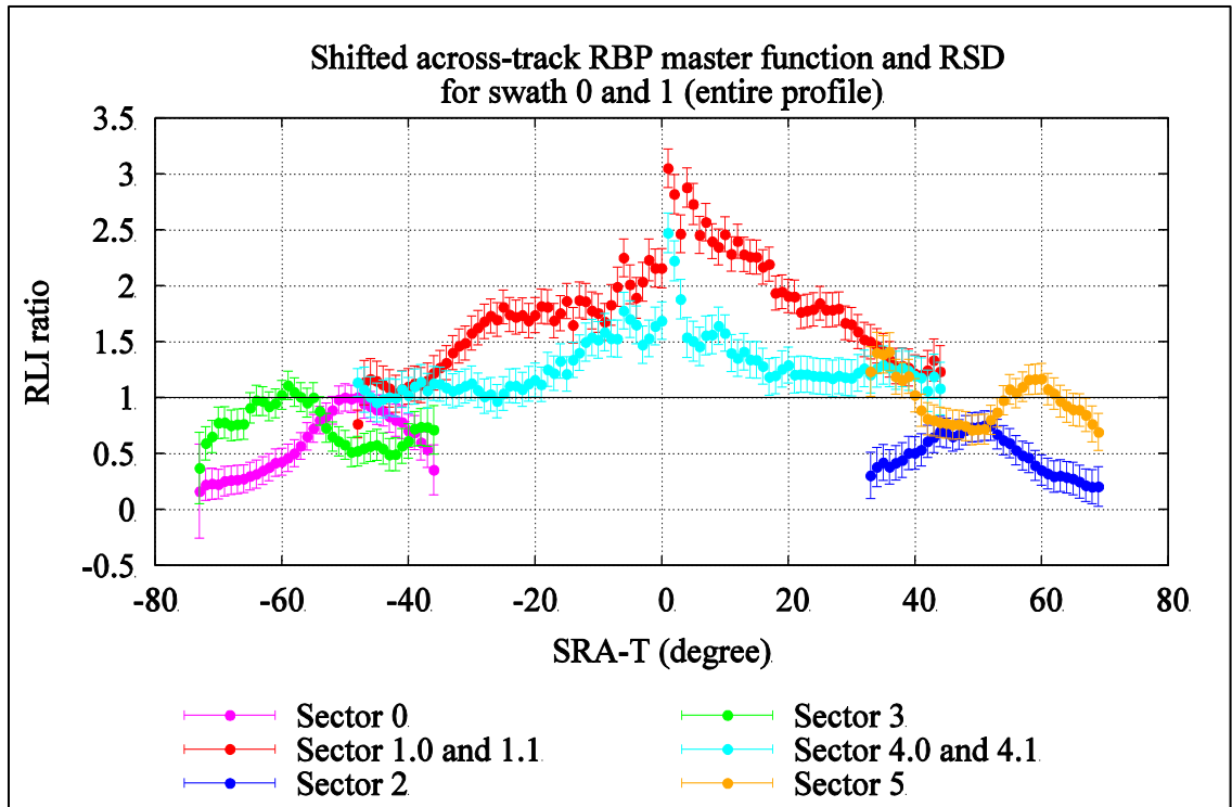
Figure 4.32: Across-track RBP master functions referenced to SRA-T -50^\circ of sector 0
