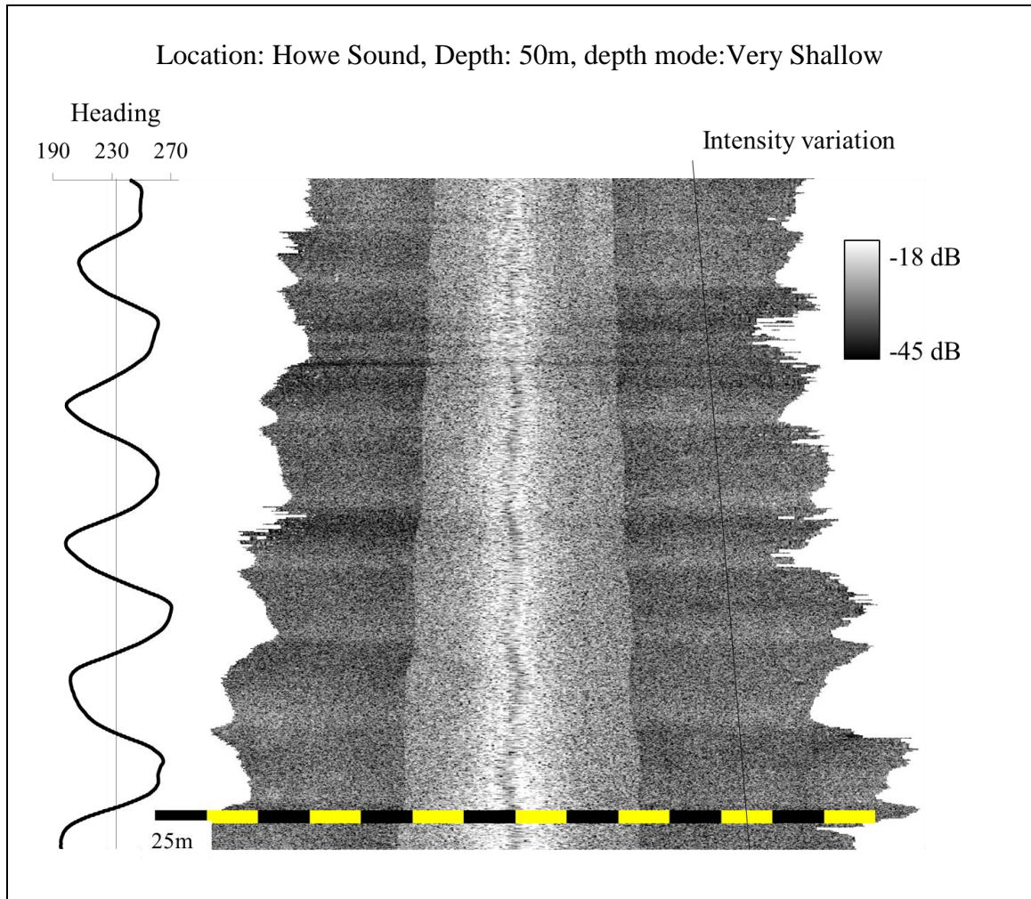
Figure 4.37: Showing received intensities for along-track RBP extraction from one of the test survey lines
