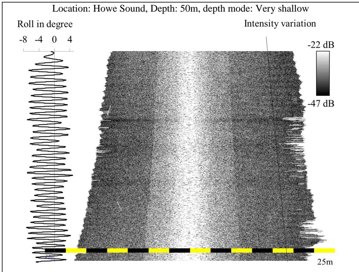
Figure 4.14: TVG-BS and geometric effect free backscatter intensities
