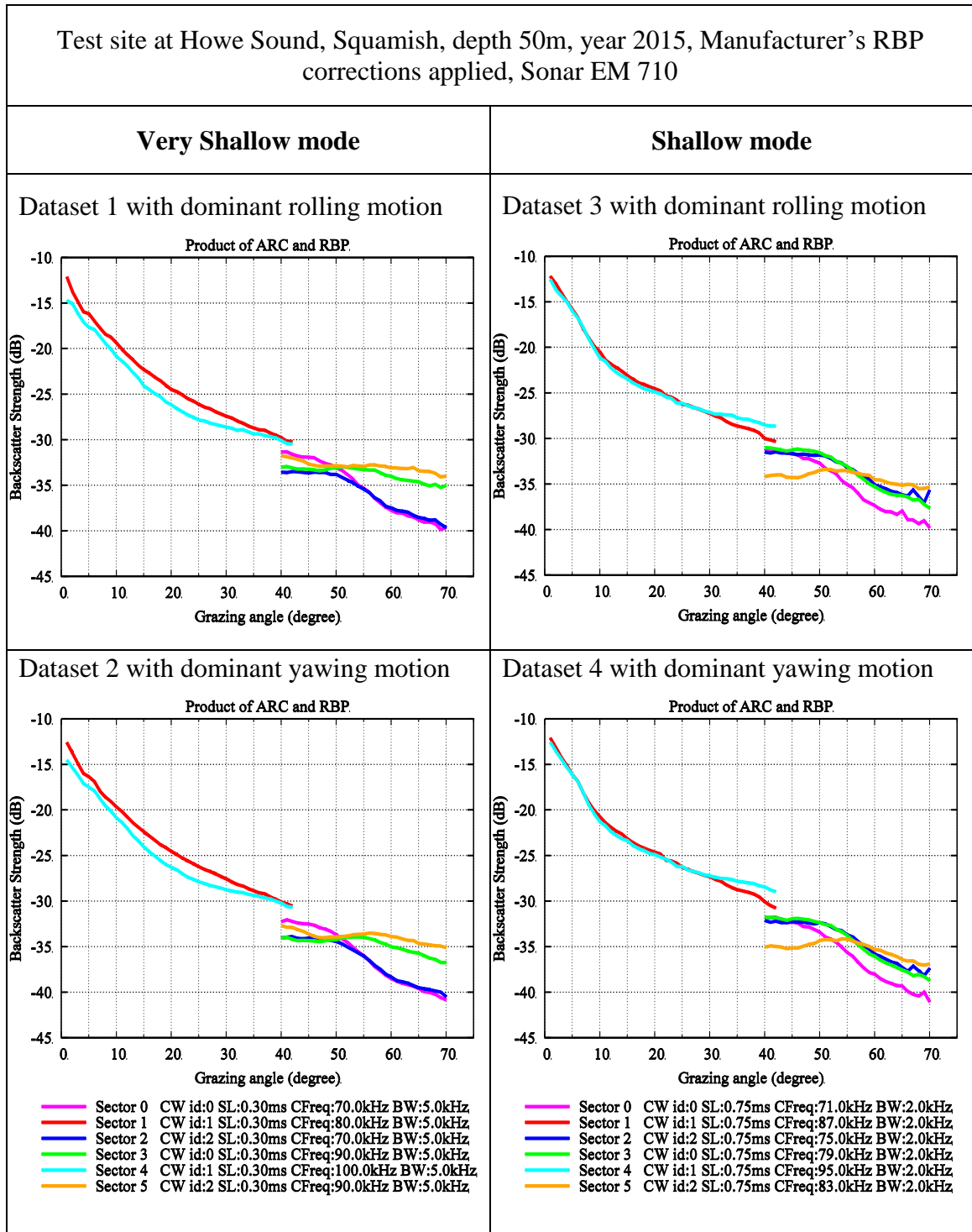
Figure 6.2: Product of ARC and RBP for cases 1, 2, 3, and 4
