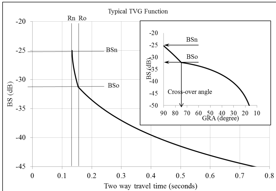
Figure 2.8: Manufacturer applied TVG to account for changing BS. The function is computed for 100m depth with crossover angle of 75°
