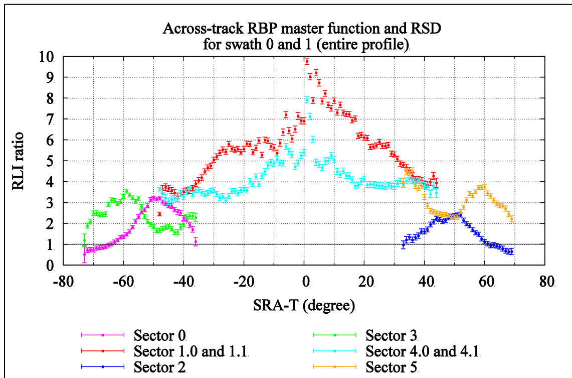
Figure 4.31: Across-track RBP master function referenced to SRA-T -63^{\circ} of sector 0
