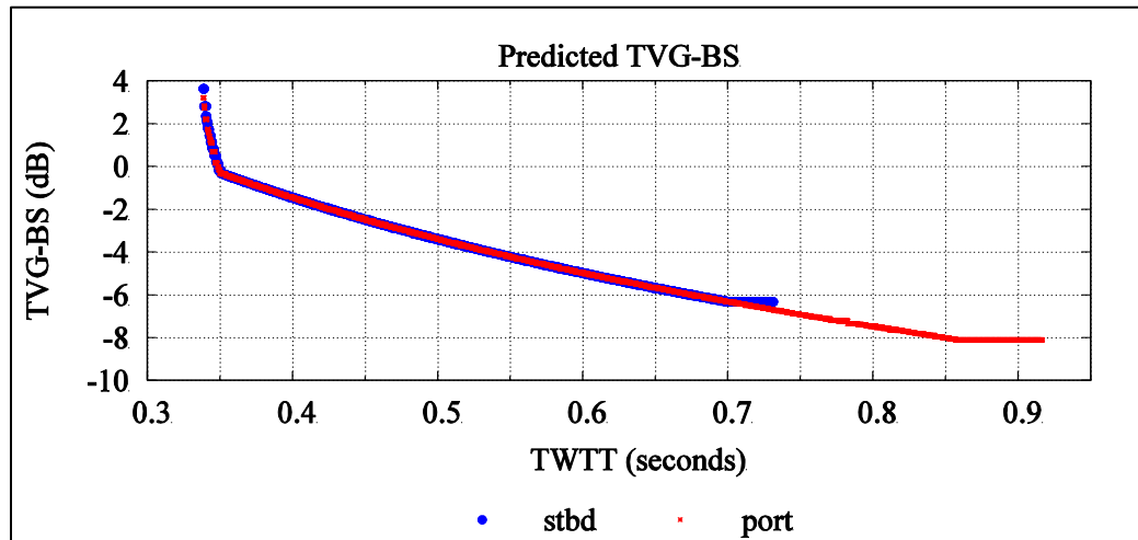
Figure 4.1: Manufacturer applied TVG-BS for a single profile.
