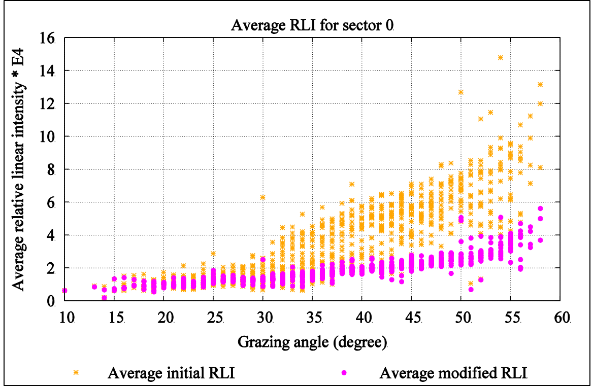
Figure 4.26: The average initial RLIs and MRLIs for sector 0
