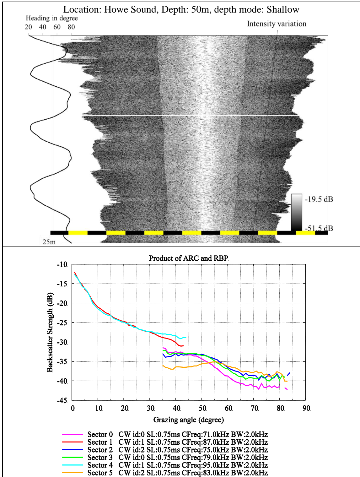
Figure 4.6: TVG-BS-free backscatter intensities for along-track RBP extraction with the product of ARC and RBP from test survey line collected in Howe Sound (Squamish)
