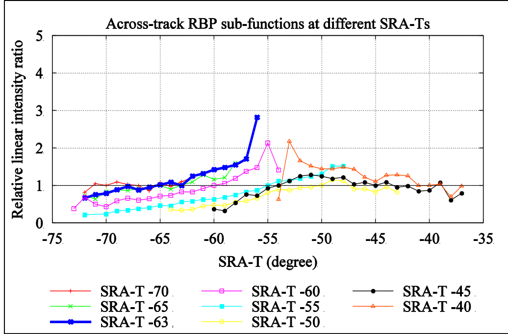
Figure 4.18: Across-track RBP sub-functions with chosen reference sub-function at SRA-T -63° for sector 0 of example dataset
