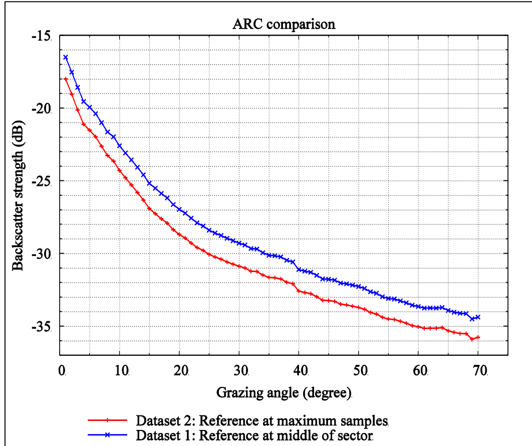
Figure 5.4: Similar ARCs with different absolute backscatter strength obtained in case 1 and 2
