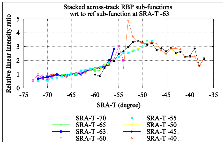
Figure 4.21: Few of the stacked sub-functions from sector 0
