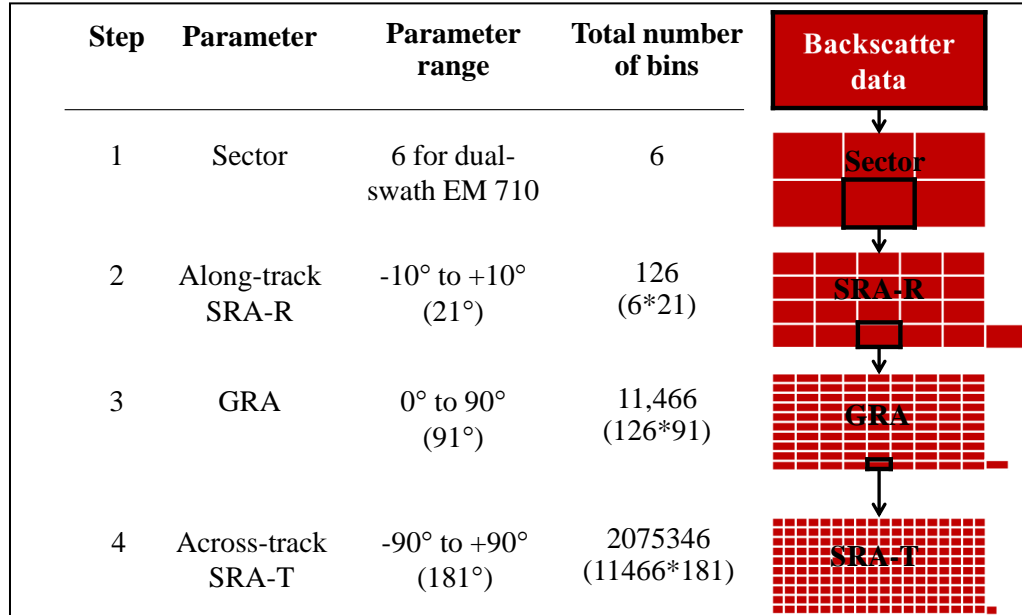
Figure 4.11: Order of backscatter data separation
