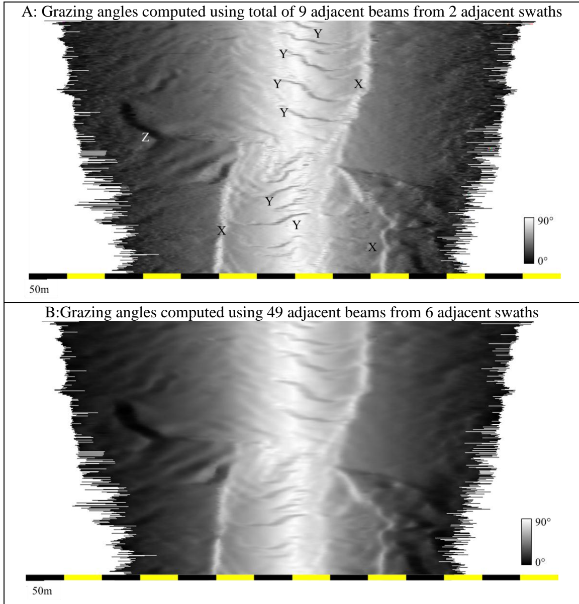
Figure 4.8: Images showing computed GRZs using different numbers of adjacent beams. X=local high GRA due to inward facing slopes, Y= low GRA near nadir due to steep along-track slope, Z= extremely low GRA due to outward facing slopes
